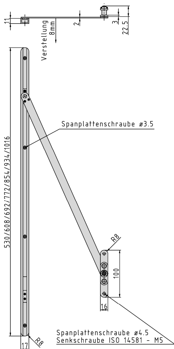
Section Drawing
